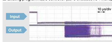
Existing programmable controller (LCPU embedded I/O + interrupts)
